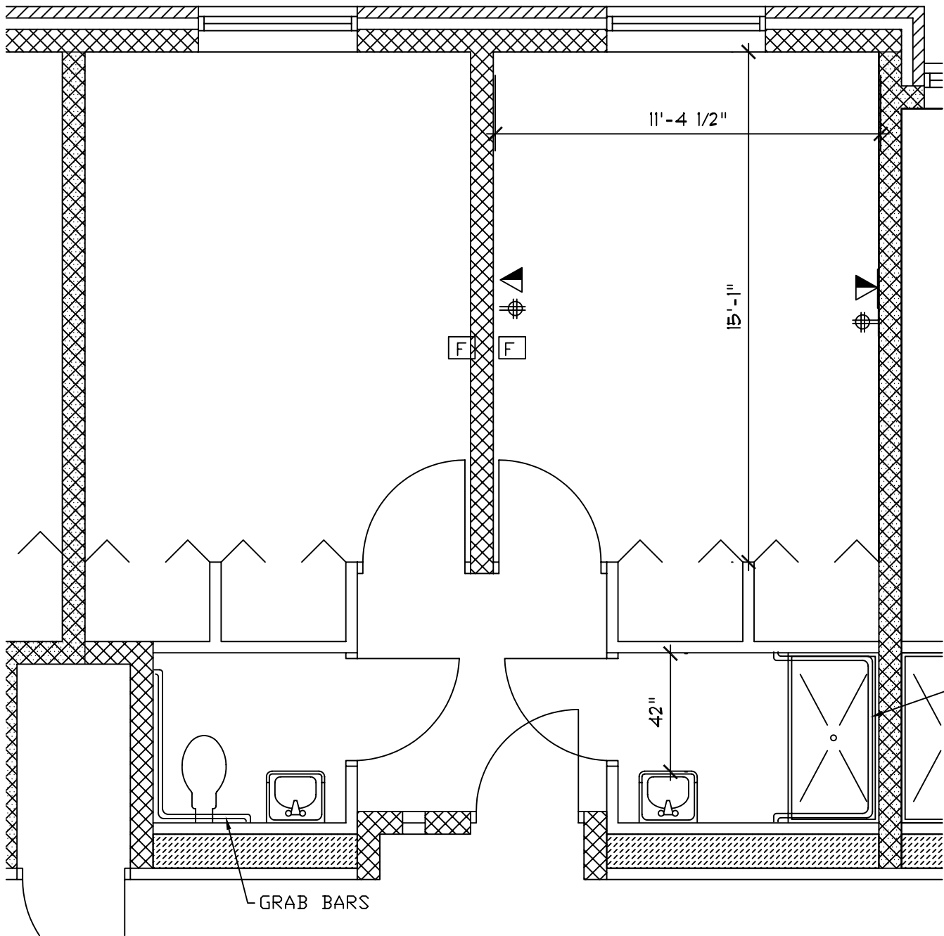
1940 RESIDENCE HALL SECOND FLOOR ROOM E213
