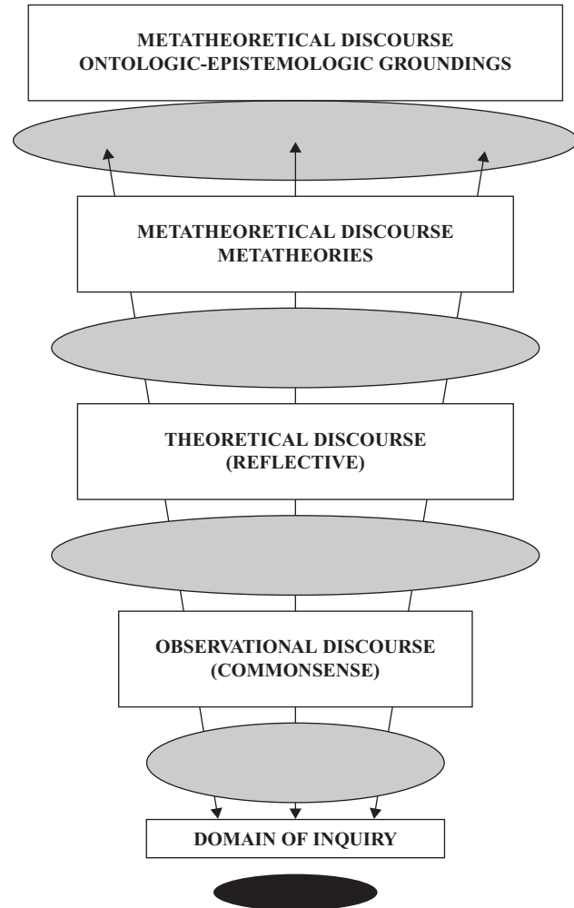
Figure 1.1 Levels of discourse.
