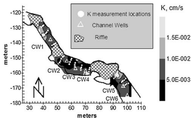
Fig. 5 Hydraulic conductivity contours of lower layer bed sediments (10–12.5 cm below the streambed)
