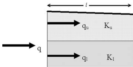
Fig. 7 Conceptual schematic of hyporheic flowpath. q is specific discharge, K is hydraulic conductivity, i is the head gradient, and subscripts u and l indicate upper and lower sediment layer, respectively. In a heterogeneous sediment with a constant head gradient, flow is divided between incremental layers based on variation in K , such that q is equal to q_u plus q_l
