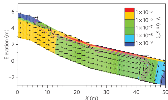
Figure 4 | Average pore-water velocity and salinity in the right transect. The averages were calculated over a spring-neap tidal cycle. The magnitude of the average pore-water velocity is reported as banded coloured contours because of its wide value range. Vectors with uniform length were used to indicate the velocity direction alone. The three solid pink curves are contours of the pore-water/seawater salinity ratio (simulated pore-water salinity divided by seawater salinity) averaged over a spring-neap tidal cycle. They are for 0.1, 0.5 and 0.9, and should be read from lower-left to upper-right.
