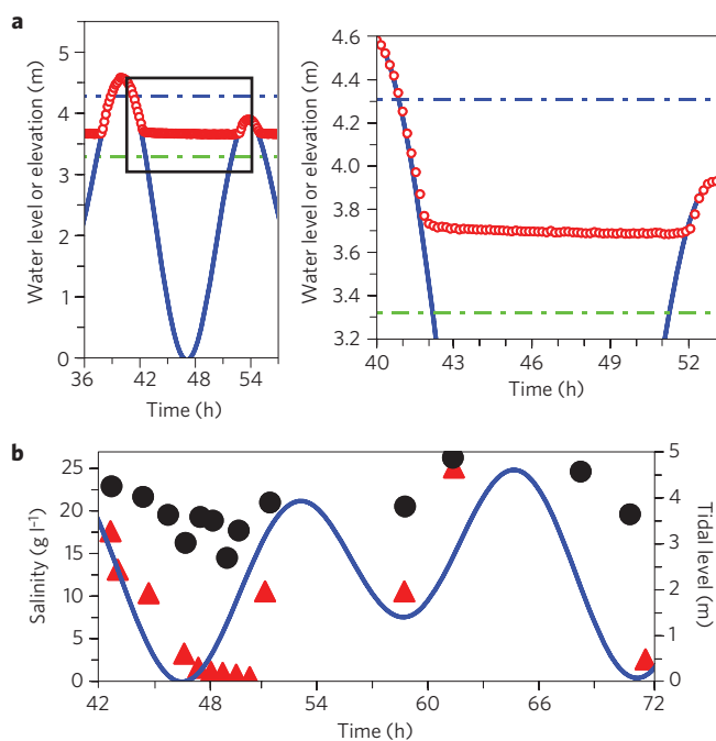
Figure 2 | Typical observations. a, b , Observed water table at R2 ( a ) and salinities at L4 and R4 ( b ). The red open circles represent the water table. The tidal level (solid blue line), and elevations of the beach surface (blue dashed line) and of the pressure transducer (green dashed line) installed at R2 are also shown. The water table fell from the surface (4.31 m) as quickly as the tide to ~3.7 m where it became almost constant. Note the decrease in salinity during the first low tide at L4 (depth 0.57 m) of the left transect (red triangles) in comparison with R4 (depth 0.54 m) of the right transect (black dots).
