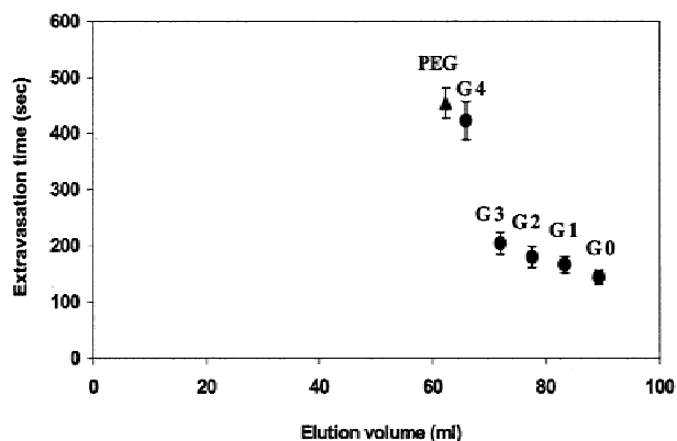
Fig. 6. The relation between extravasation time ( \tau ) (s) and the elution volume of polymers on a Superose 12 HR 16/50 preparative scale column (Amersham Pharmacia Biotech) following the experimental conditions reported in the experimental methodology section. (●), PAMAM dendrimers; (▲), PEG.
