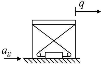
Fig. 1. SDOF Building
