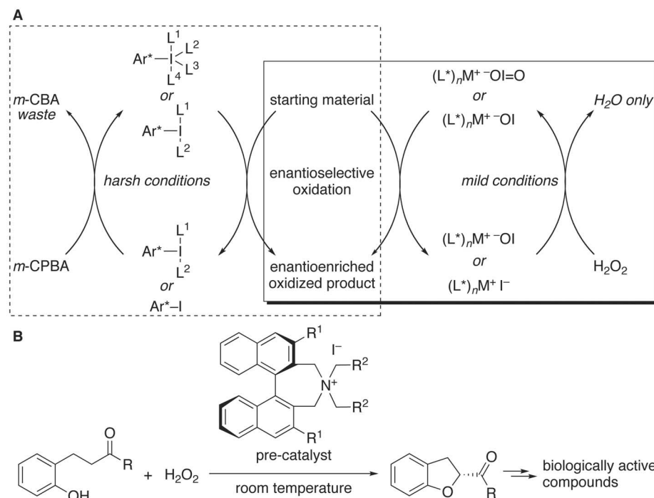
Fig. 1. (A) (Left) Known in situ-generated aryl- \lambda^3 - or aryl- \lambda^5 -iodane catalysis. (Right) In situ-generated hypiodite(I) or iodite(III) catalysis. (B) Design of inorganic iodide pre-catalyst paired with a chiral quaternary ammonium counter ion for the enantioselective oxidative cycloetherification of ketophenols to 2-acyl-2,3-dihydrobenzofuran derivatives. Ar, aryl; L, ligand; M + , metal or onium cation, R, alkyl or aryl group. Symbols (Ar and L) marked with asterisks represent chiral groups.
