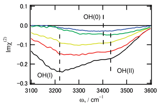
Figure 3. The complex \chi^{(2)} spectra of airy interfaces of aqueous 0.1\text{ mM} CTAB solutions at various isotopic concentrations (black, \text{H}_2\text{O} ; red, \text{H}_2\text{O}/\text{HOD}/\text{D}_2\text{O} = 9:6:1 ; yellow, 1:2:1 ; green, 1:6:9 ; blue, 1:12:33 ). The SF, \omega_1 , and \omega_2 beams were s -, s -, and p -polarized, respectively.
